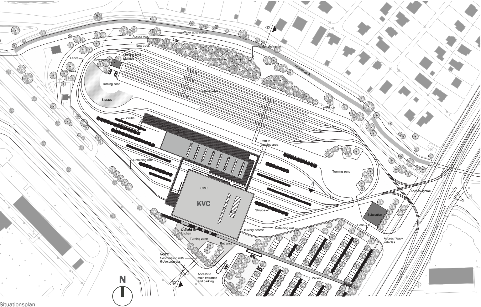
Situationsplan
